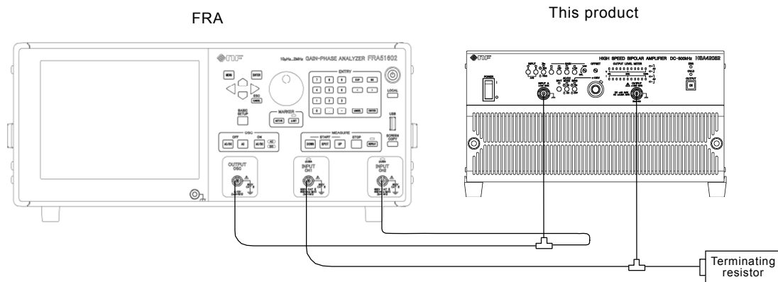
Figure 6-4. Measurement of Frequency Characteristics
