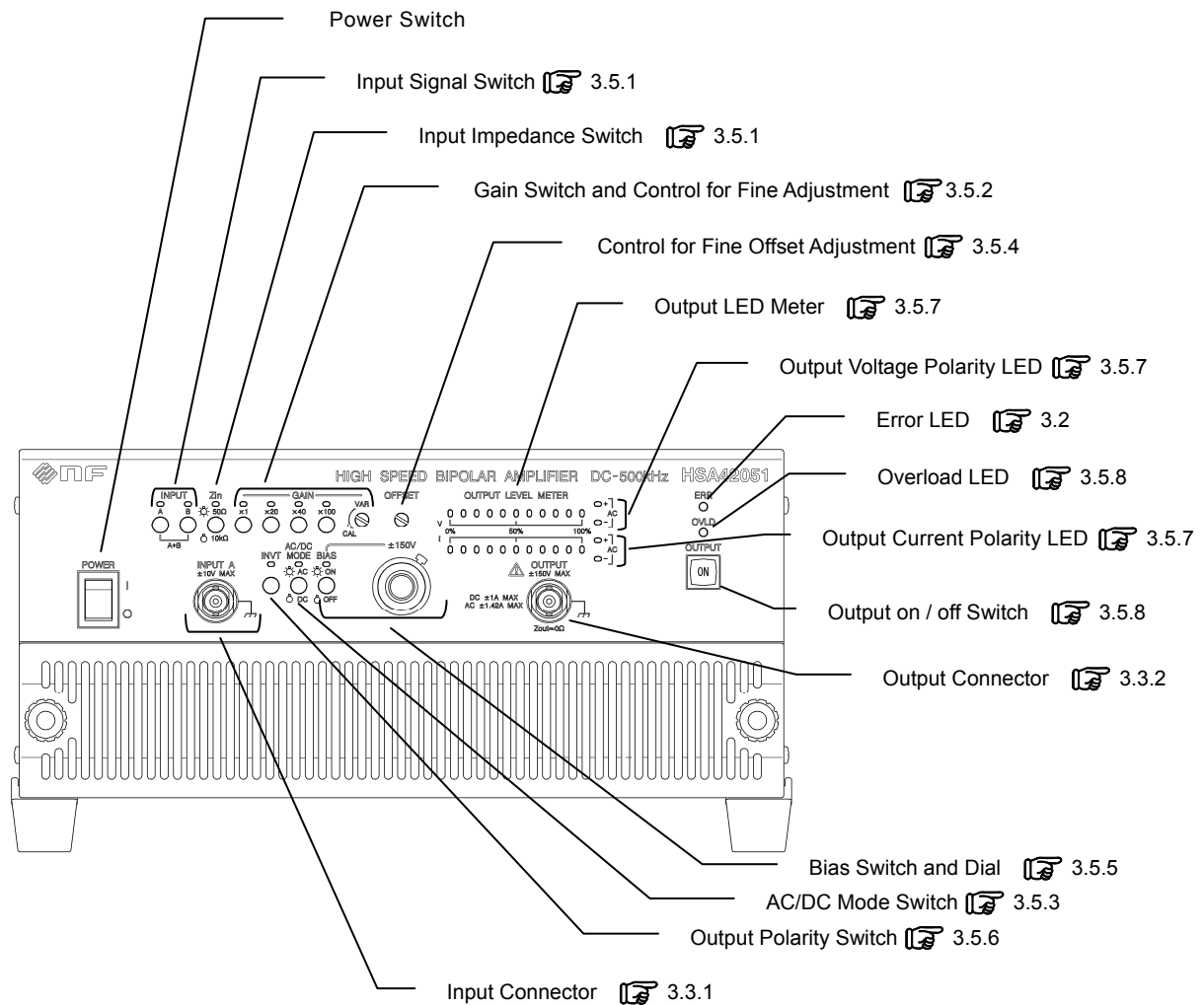
Figure 3-1. HSA42051 Front Panel
