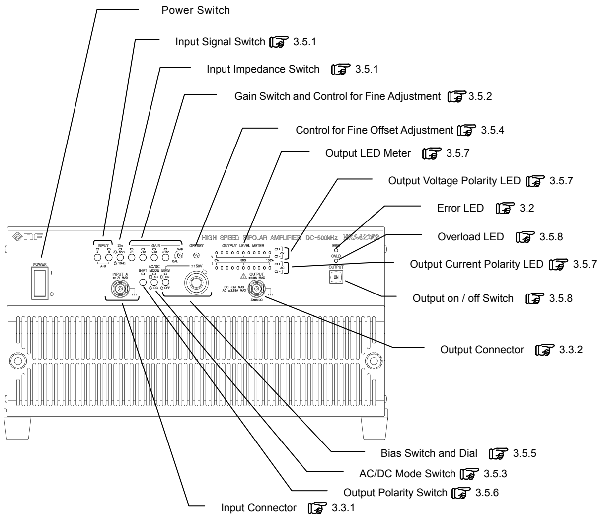
Figure 3-2. HSA42052 Front Panel
