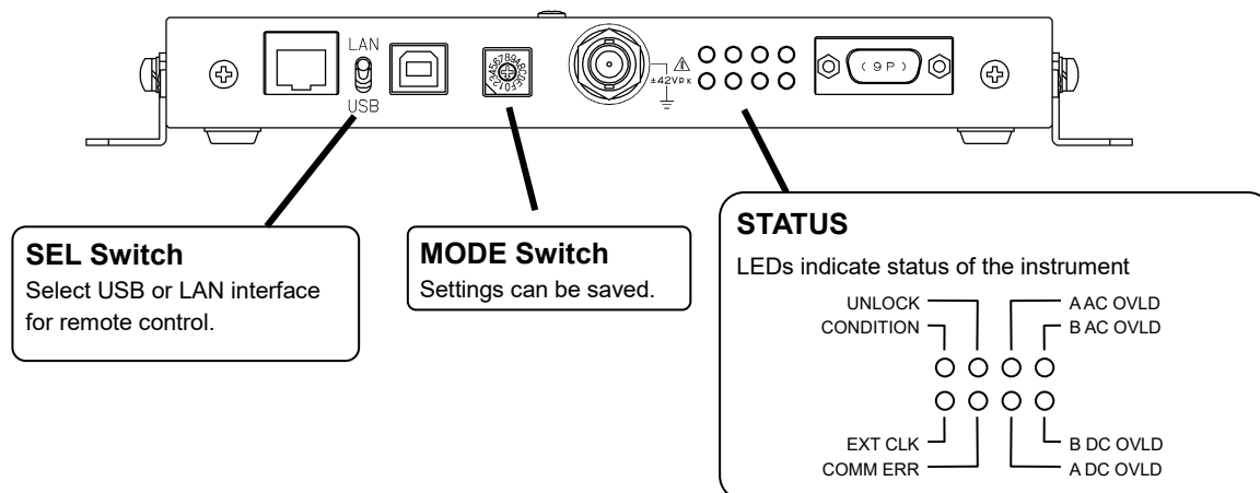
Figure 3-2 Rear side
