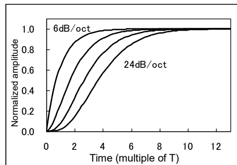
Step response waveform
