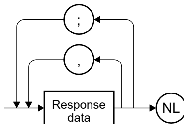
Figure 5-14 Response message syntax
