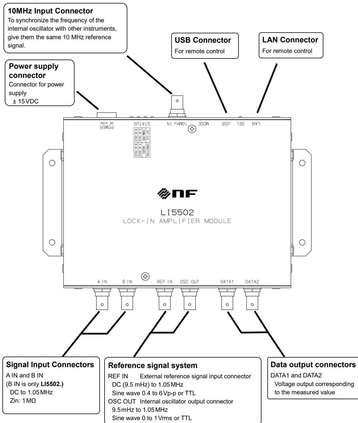
Figure 3-1 Top side
