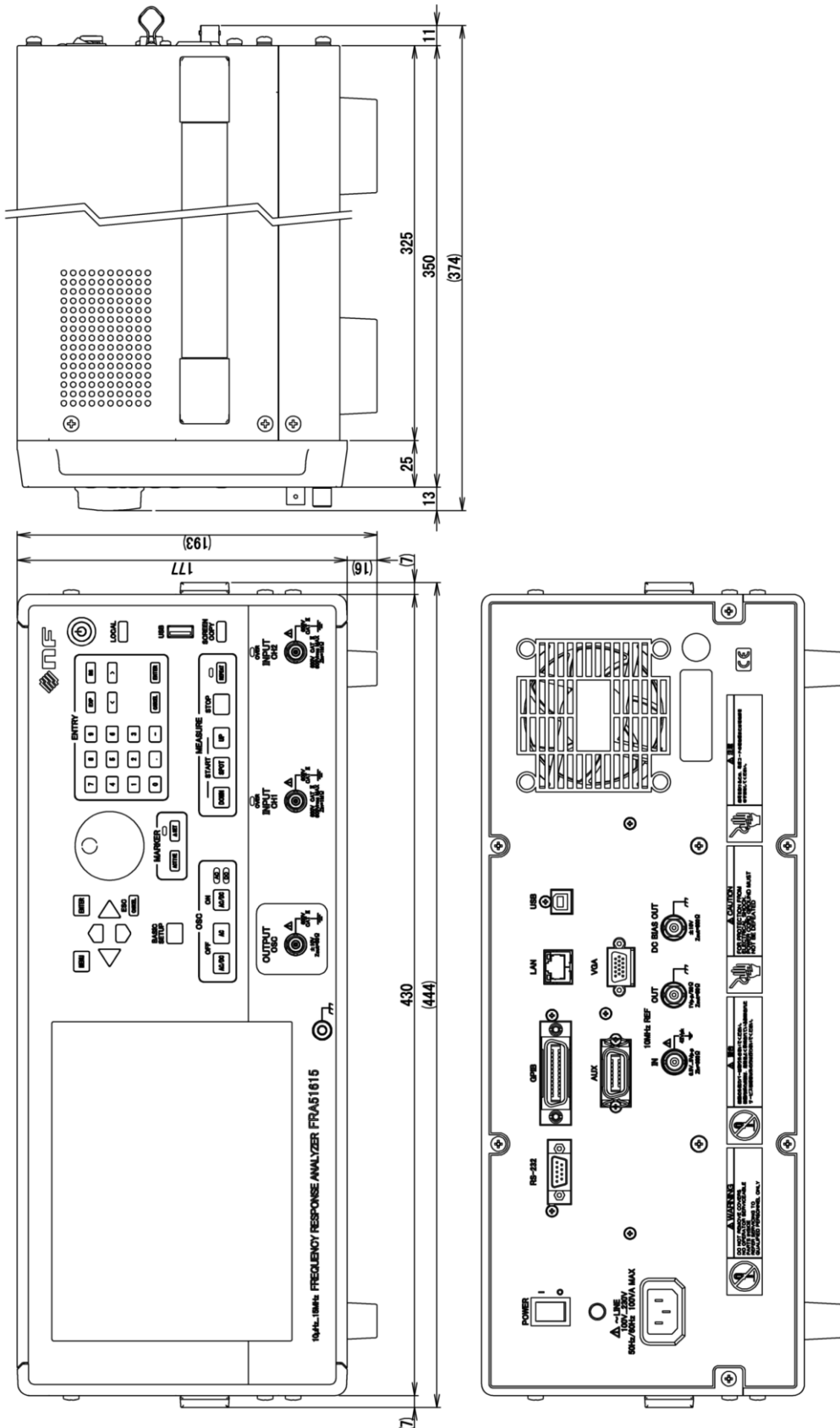
Figure 1-3 External dimensions
