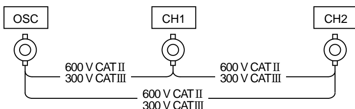
Figure 1-2 Isolation voltage specifications between signal connectors
