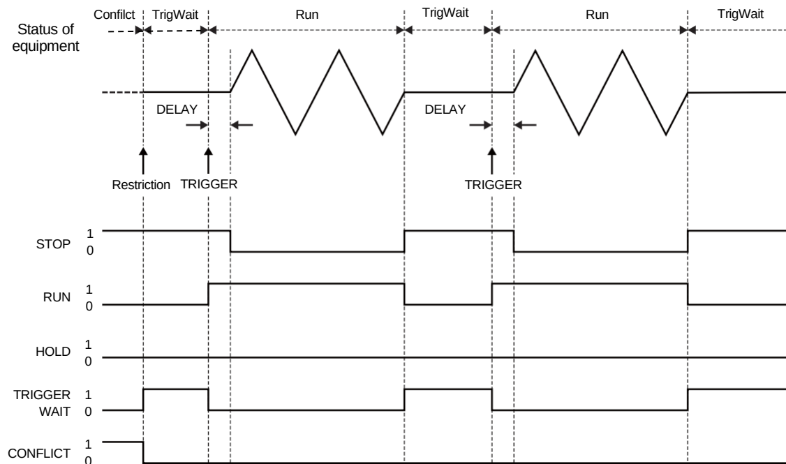
Figure 3.9 Relationship between Output and Operation Status Register (Bit 7 to 11) at Trigger Burst
