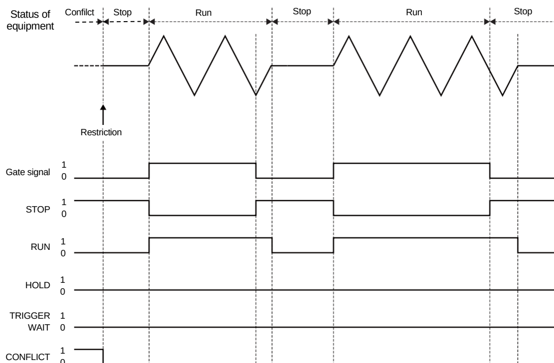
Figure 3.10 Relationship between Output and Operation Status Register (Bit 7 to 11) at Gate
