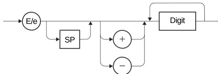
Figure 2.6 Index Syntax
